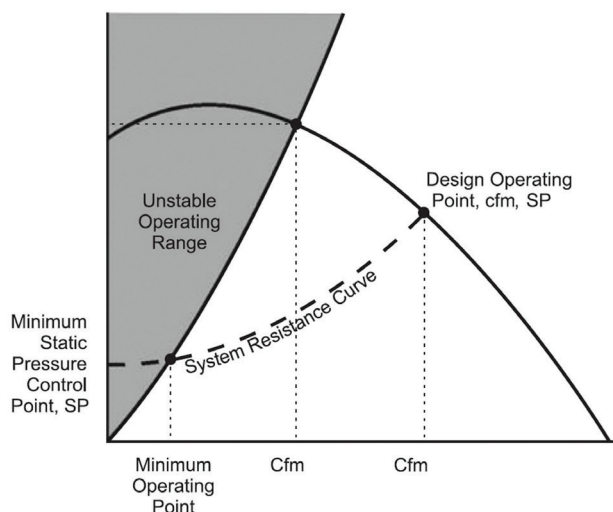
Figure 18: Variable Air Volume (VAV) Control
