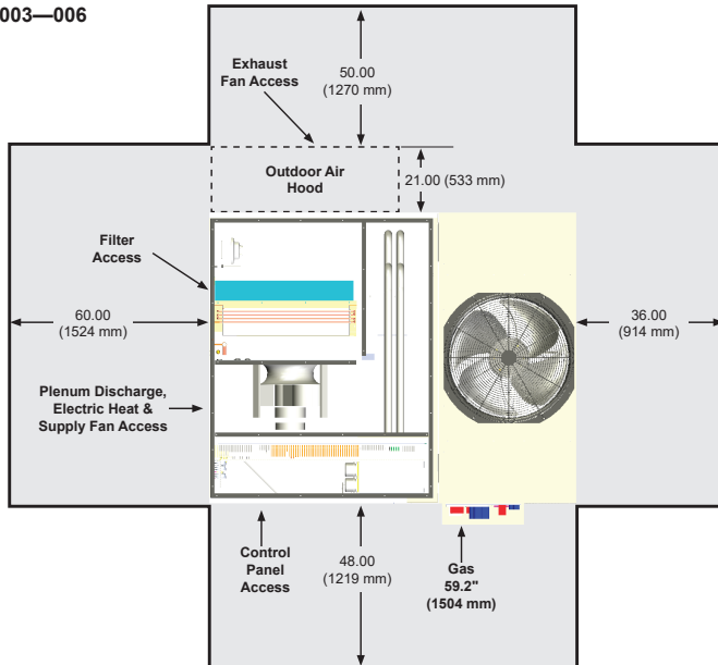
Figure 13: Service Clearances
