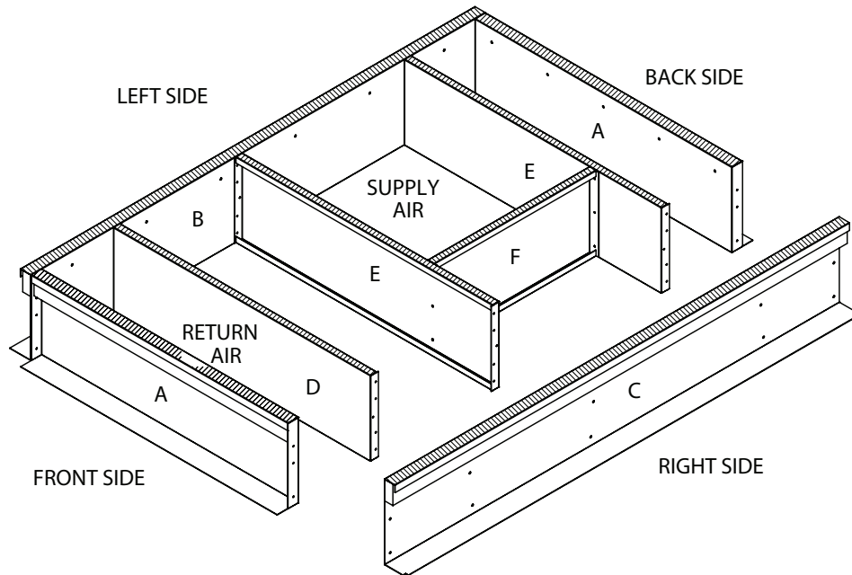
Figure 15: Roof Curb Assembly (DPS 007-015)¹
